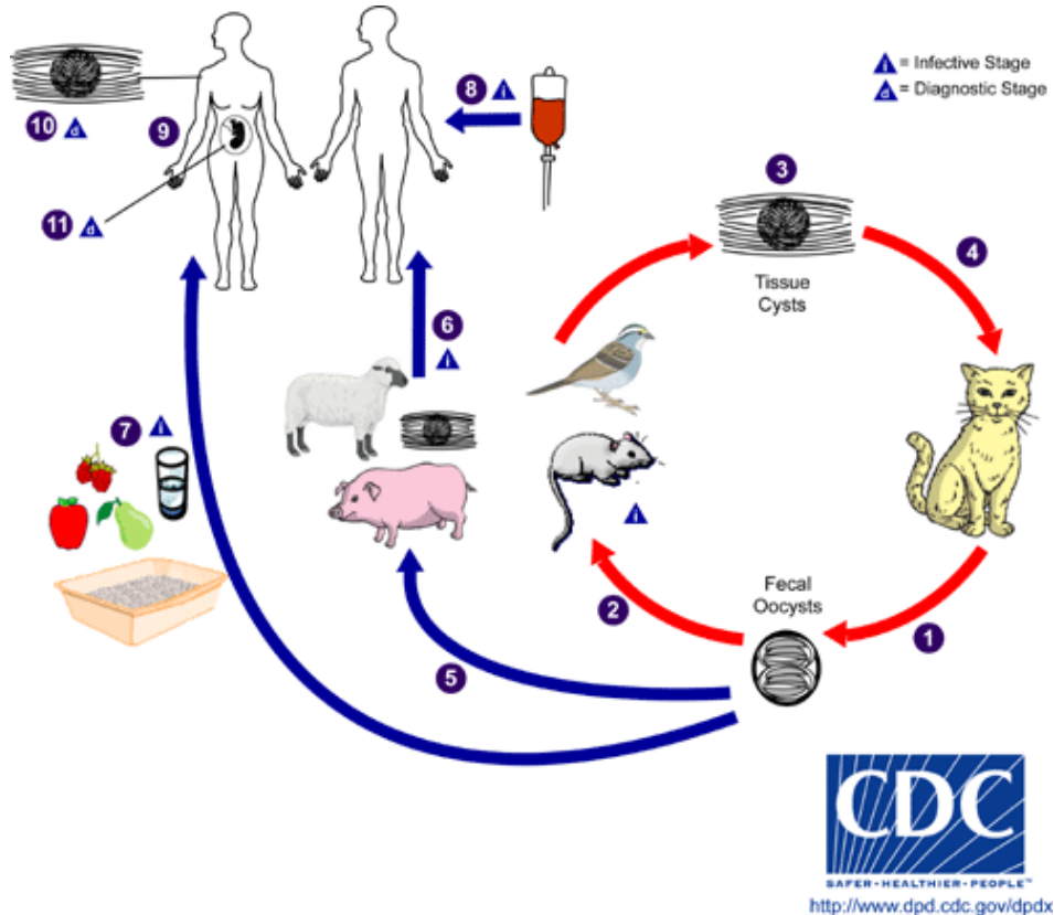
Figure TO1. Life cycle of Toxoplasma gondii
