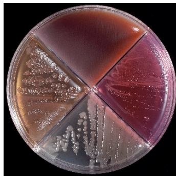
Proteus mirabilis
