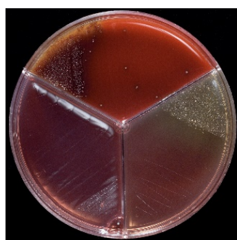
Enterococcus spp.
