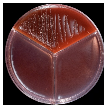
Streptococcus uberis
